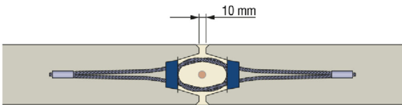
Fig. B.16: Minimal joint
