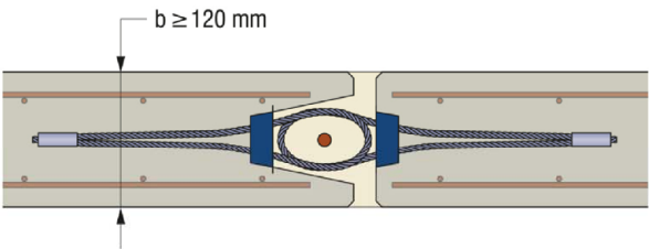
Fig. B.8: Wall – Wall connection ( flat installation )
