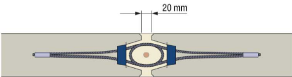
Fig. B.15: Standard joint
