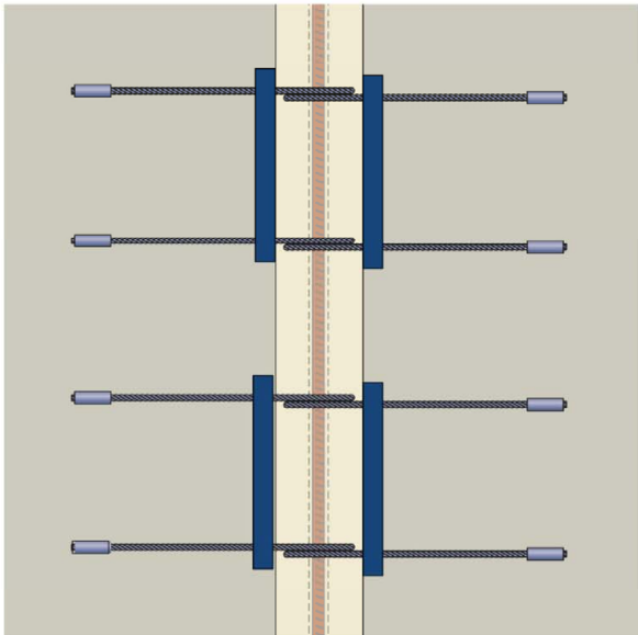
Fig. B.18: Standard wire loop overlap
