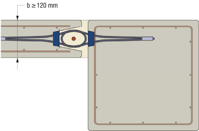
Fig. B.9: Column – Wall connection ( flat installation )
