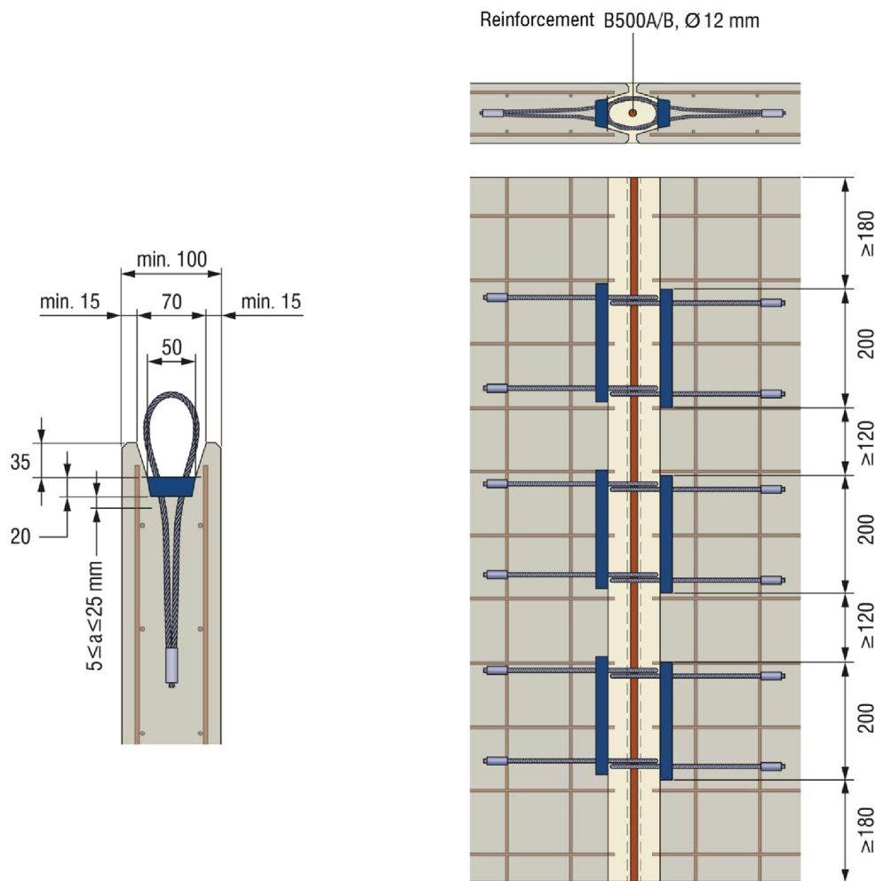
Fig. B.7: Geometry, reinforcement (Detail precast element A and B)
