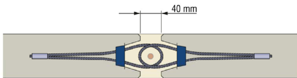
Fig. B.17: Maximal joint
