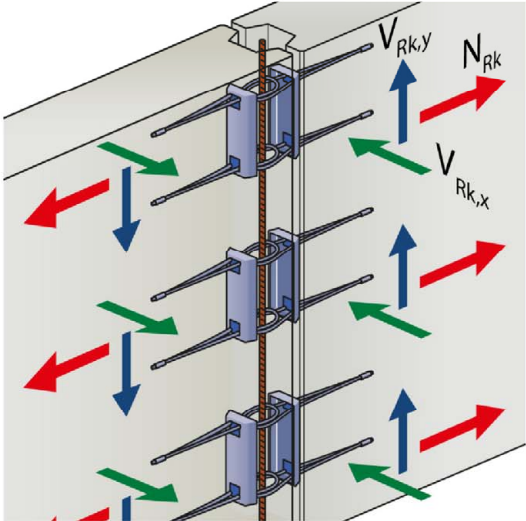
Fig. C.4: Load combination
