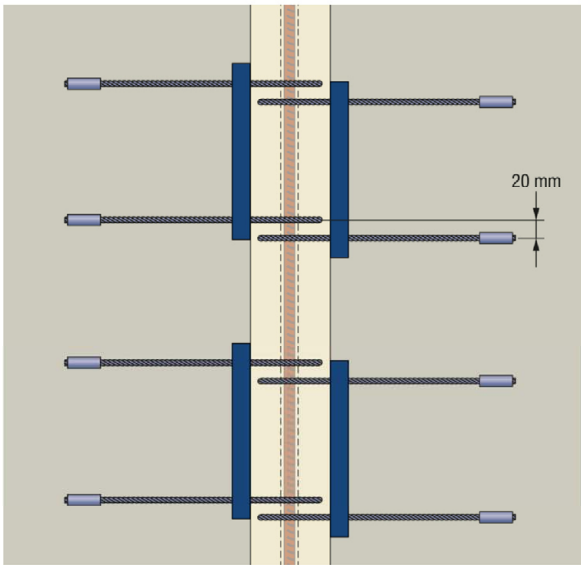
Fig. B.19: Maximal vertical tolerance: 20 mm
