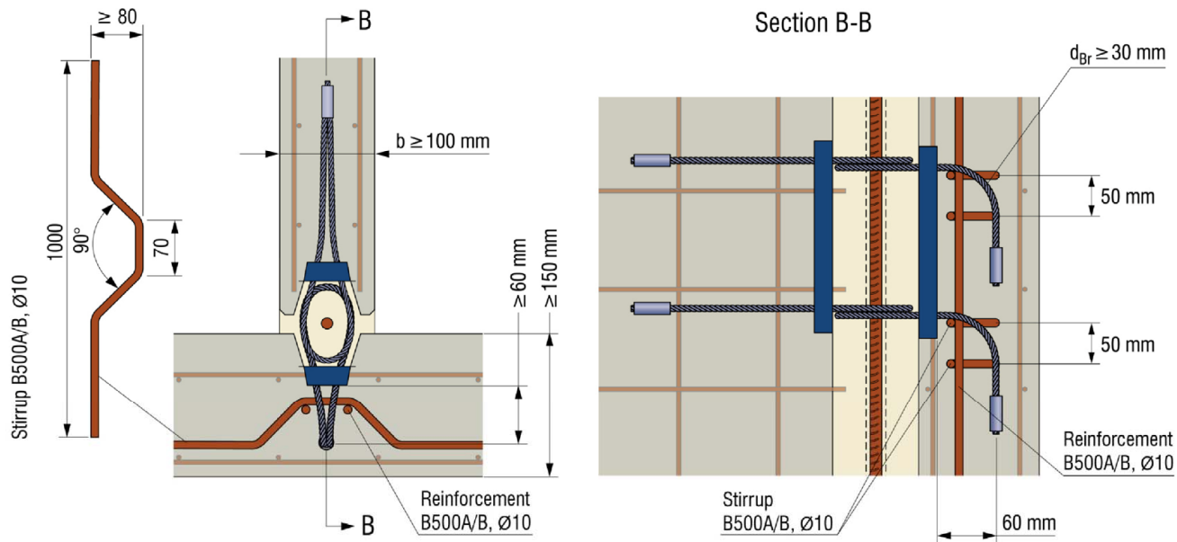
Fig B.6: Wall – Wall – T-Connection - Detail with bended wire loops
