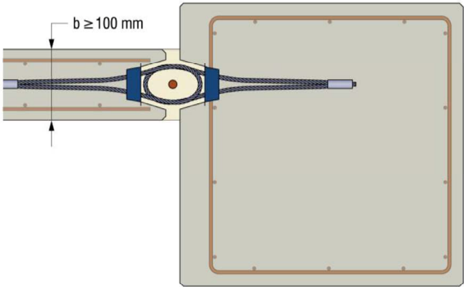
Fig. B.2: Column – Wall connection ( recessed installation )
