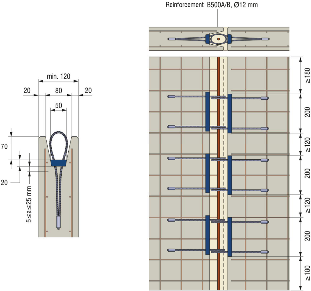
Fig. B.14: Geometry, reinforcement (Detail precast element A and B)
