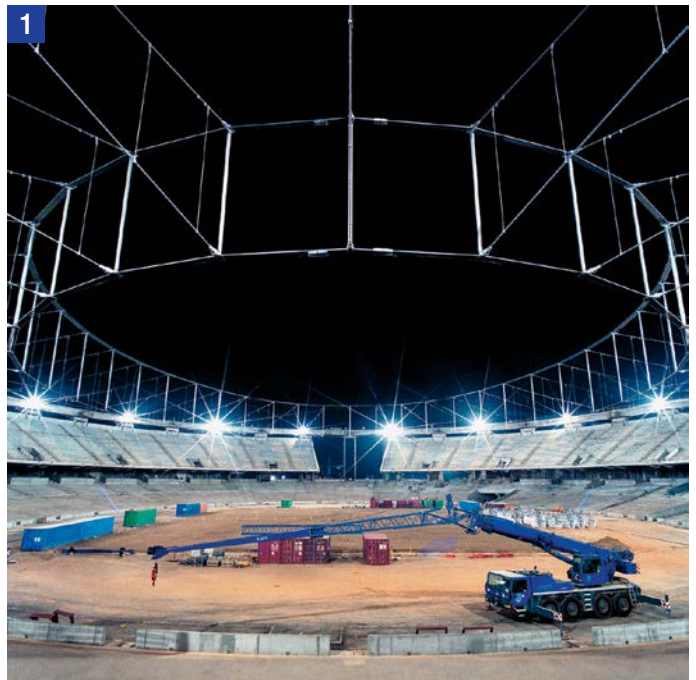
1 Prestressed cable structure before membrane installation
