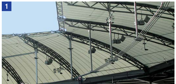
1 Ring cable with lower radial cables and upper steel girders
