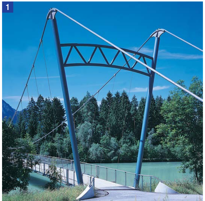
1 Pylon head with suspension cables
