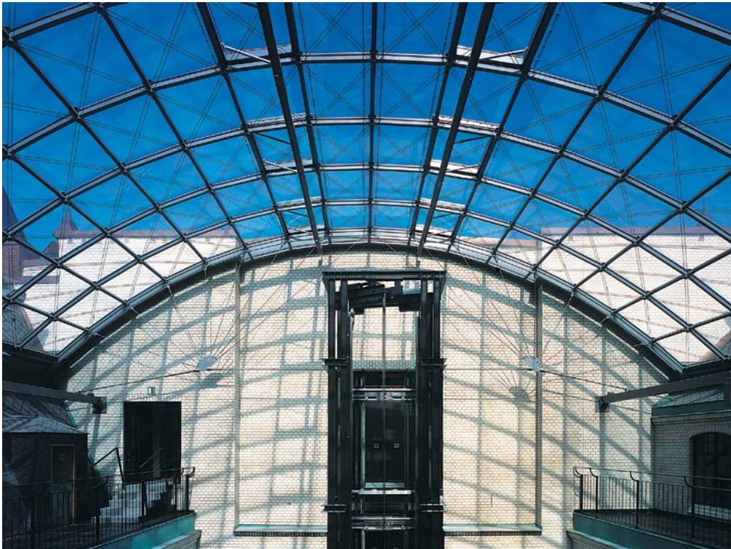
1 Spider cables as bracing of roof structure
